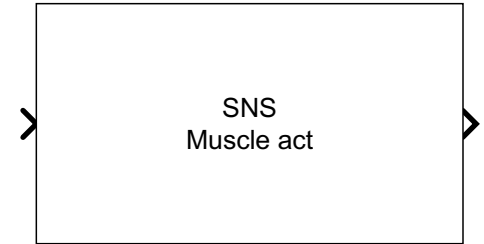
MuscleActivation
